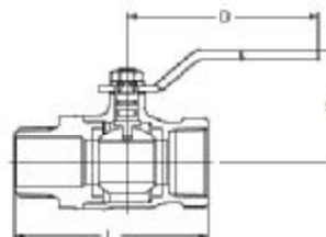
Dimensions of TO
