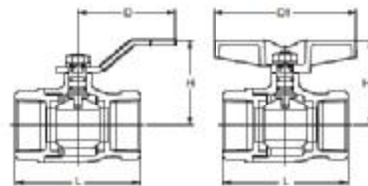
Dimensions of T, TT, AKT
