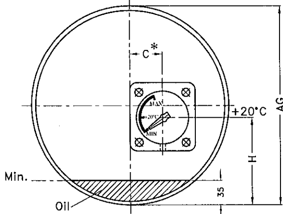
Mounting for conservator
