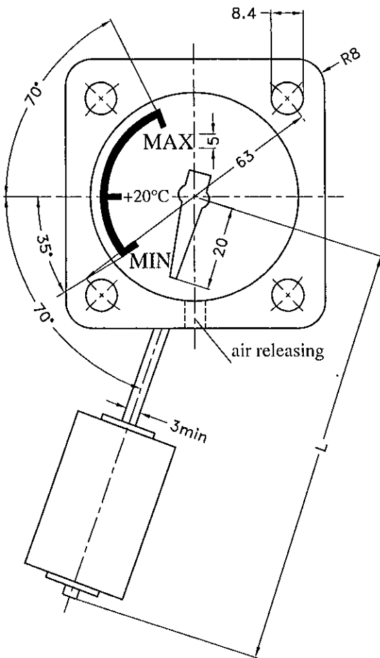
Mounting for conservator
